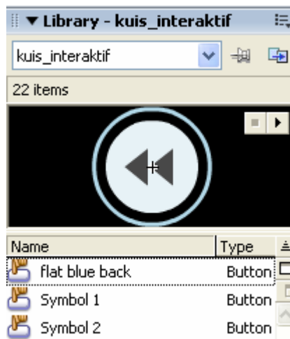
Gambar 1.6: Panel Library
